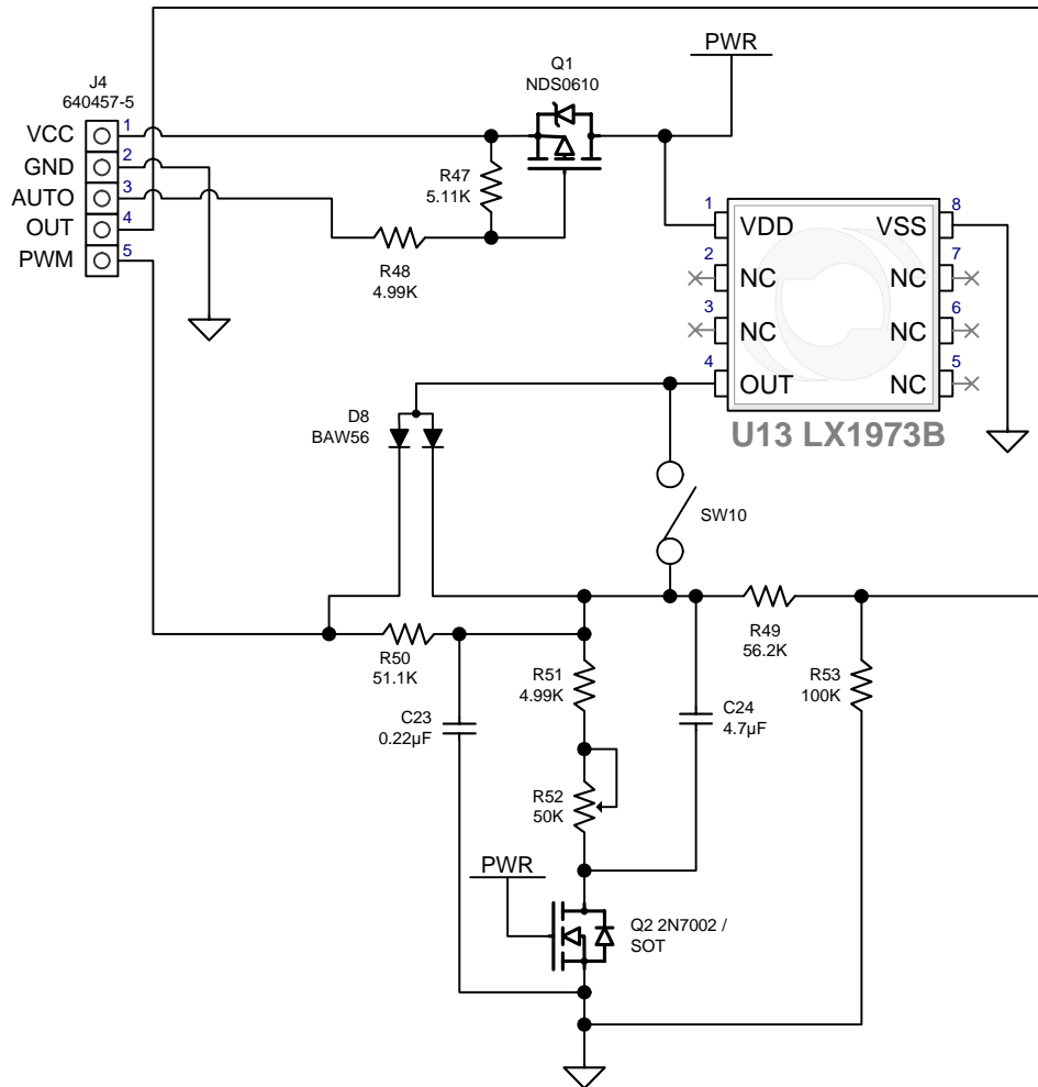
Figure 1 - LX1973B Evaluation Board Schematic
